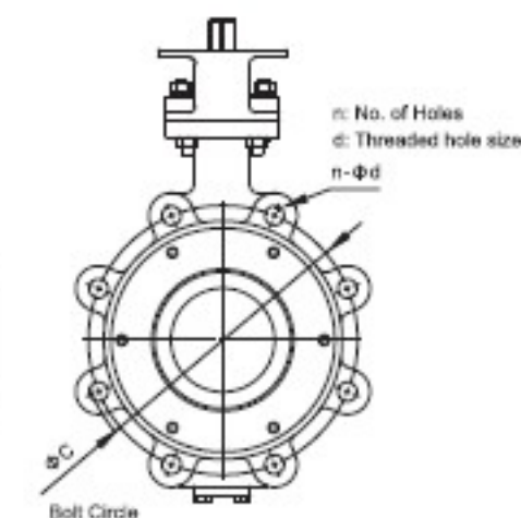
121L Lugged Body Style
