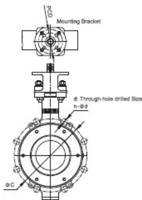
121W Wafer Body Style
