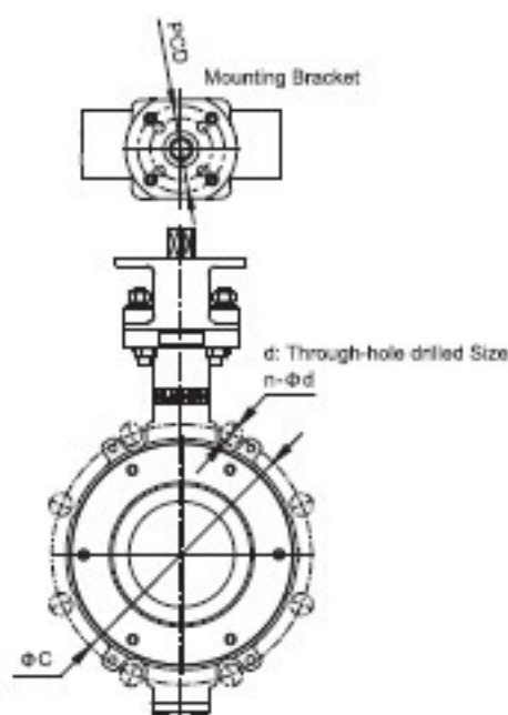
122W Wafer Body Style
