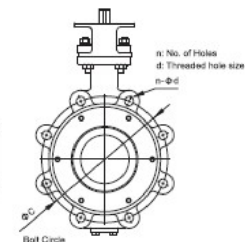
122L Lugged Body Style
